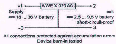
Fig. 4: block diagram A WE X 020 A01
