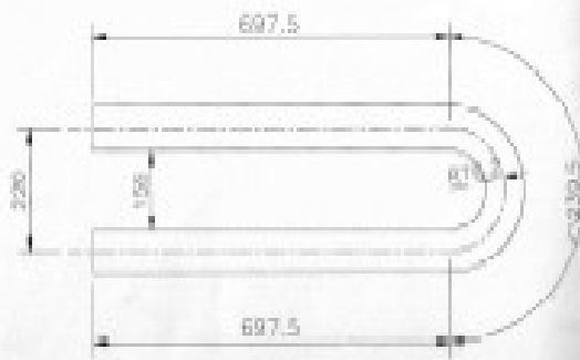
STYLE - 1 REHEATER COIL BEND
