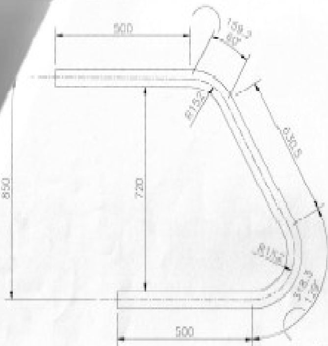
STYLE - 4 REHEATER COIL BEND
