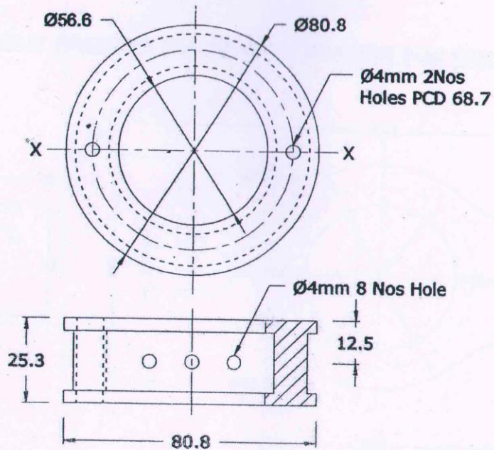
SECTION X-X
