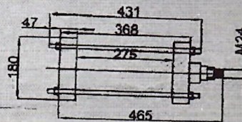
Power Cylinder for 200 mm Gate Valve
